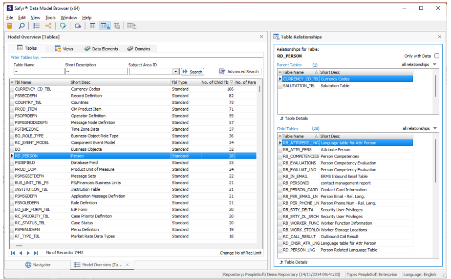
Example screenshot of Person table and related tables from Safyr for PeopleSoft
